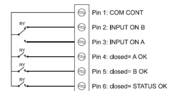
Contacts port basic diagram
